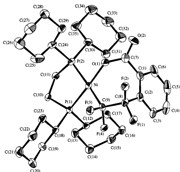
Fig. 3 An ORTEP diagram for [\text{Ni}\{\text{OC}(\text{O})\text{C}_6\text{H}_4\text{CF}_2\text{CF}_2\text{-}2\}(\text{dcpe})] \mathbf{16} with atom labelling and 20% probability ellipsoids
