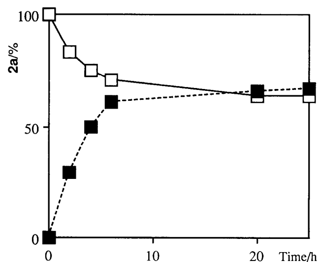
Fig. 2. Isomerization of 2a and 2b at 80°C, (□) Start from 2a ; (■), start from 2b . Initial concentration, 2.7 \times 10^{-2} mol dm -3 in CD 3 C 6 D 5 .
