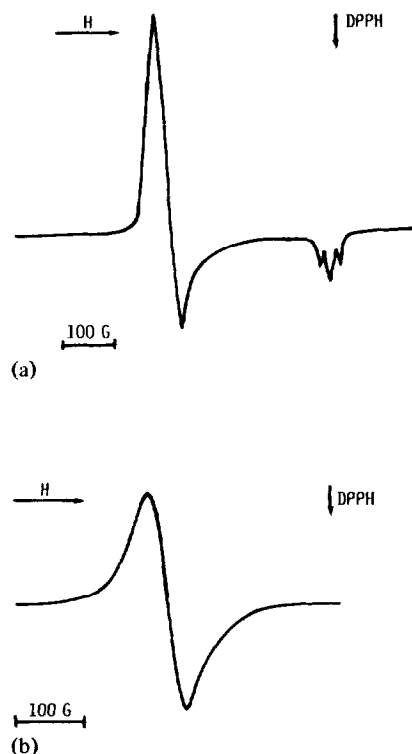
Fig. 2. X-band ESR spectra of the electrochemically generated monocation [2]^+ in CH_2Cl_2 – [NBu_4]ClO_4 (0.1 mol dm^{-3} ): (a) 100 K; (b) 300 K.
