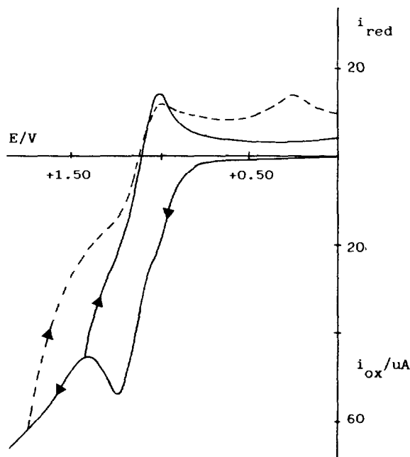
Fig. 3. Cyclic voltammogram recorded at a platinum electrode on a \text{CH}_2\text{Cl}_2 solution containing \text{Rh}_2(\text{COD})_2(\text{O}_2\text{CCH}_3)_2 ( 2.3 \times 10^{-3} \text{ mol dm}^{-3} ) and [\text{NBu}_4]\text{ClO}_4 ( 0.1 \text{ mol dm}^{-3} ). Scan rate 0.2 \text{ V s}^{-1} .
