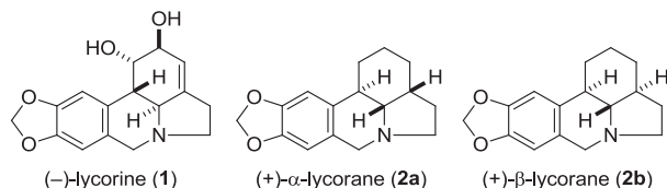
Fig. 1. Structures of lycorine and lycoranes.
