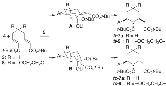
Scheme 2. Rationale for observed diastereoselectivity.
