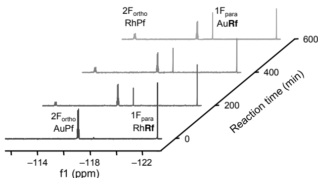
Figure 1. Reaction between [AuPf(AsPh 3 )] (1) and trans -[RhRf(CO)(AsPh 3 ) 2 ] (2) in THF at 294 K, monitored by 19 F NMR until 40% conversion.
