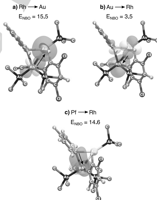
Figure 5. Isosurfaces (isovalue = 0.05 \text{ e}^- \text{ bohr}^3 ) of selected NBOs in TS1 . Above: a)+b) electron-donation between Rh and Au to form the Rh–Au bond; it can alternatively be defined as Rh-to-Au donation (a) + Au-to-Rh back-donation (b). Below: c) electron donation from the Pf group forming the C–Rh bond, while breaking the C–Au bond. Donor-acceptor interactions in each NBO, E_{\text{NBO}} (in \text{kcal mol}^{-1} ), obtained from second order perturbation theory (SOPT) are also presented. H atoms are omitted and \text{AsPh}_3 is drawn as \text{AsC}_3 for better observation.
