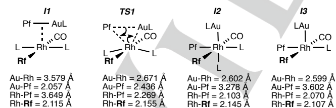
Figure 4. Evolution of bond distances along the reaction pathway. Sum of covalent radii: Au–Rh = 2.78 Å; Au–C = 2.09 Å; Rh–C = 2.15 Å.
