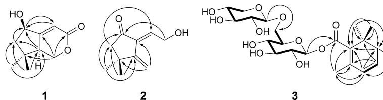
Fig. 2. Key HMBC (H → C) and COSY (H → H) correlations of 1–3
