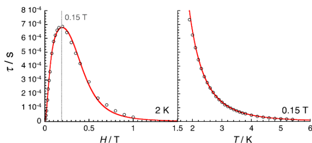
Figure 9. Field (left, at 2 K) and temperature (right, at 0.15 T) dependences of the average relaxation time for [\text{Fe}(\eta^5\text{-C}_5\text{Me}_5)_2]\text{BAr}_\text{F} estimated from Figures 4 and 5 . The red lines are the best fits obtained with the theoretical approach developed in the text using Equation 2 (without the QTM term).
