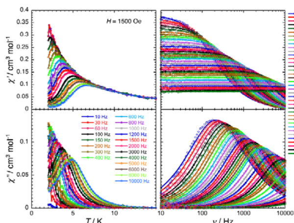
Figure 5. Temperature (left) and frequency (right) dependences of the real ( \chi' , top) and imaginary ( \chi'' , bottom) components of the ac susceptibility, between 1.9 and 15 K and between 10 and 10000 Hz respectively, for [\text{Fe}(\eta^5\text{-C}_5\text{Me}_5)_2]\text{BARf} in a 1500-Oe dc field. Solid lines are visual guides on the left part of the figure; they are the best fits of the experimental data to the generalized Debye model (see Supporting Information) on the right part of the figure.
