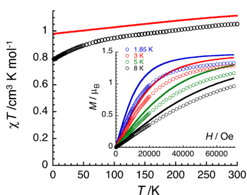
Figure 3. Temperature dependence of the \chi T product at 0.1 T for [\text{Fe}(\eta^5\text{-C}_5\text{Me}_5)_2]\text{BAR}_\text{F} ( \chi is defined as magnetic susceptibility equal to M/H per mole of [\text{Fe}(\eta^5\text{-C}_5\text{Me}_5)_2]\text{BAR}_\text{F} ). Inset: field dependence of the magnetization below 8 K for [\text{Fe}(\eta^5\text{-C}_5\text{Me}_5)_2]\text{BAR}_\text{F} (8–280 mT min -1 ). Solid lines are simulations using the NEVPT2 results discussed in the text (see Electronic Structure Calculations section).
