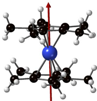
Figure 7. Representation of the NEVPT2 calculated g_z component of the \mathbf{g} -tensor for [\text{Fe}(\eta^5\text{-C}_5\text{Me}_5)_2]^+ . The z eigen-direction of the \mathbf{g} -tensor is almost perpendicular to the (\eta^5\text{-C}_5\text{Me}_5) planes (i.e., aligned with the \text{C}_5 axis).
