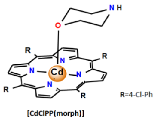
Scheme 1. Structure of [\text{Cd}(\text{TCIPP})(\text{morph})] ( I ).
