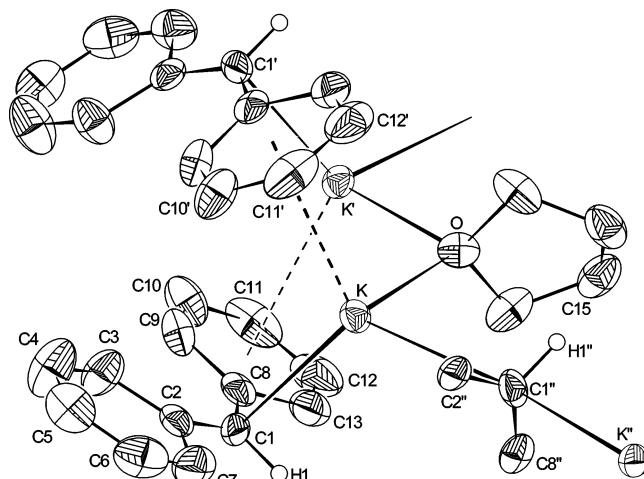
Figure 1. Molecular structure of [1(THF)_{0.5}]_\infty (30% probability thermal ellipsoids); hydrogen atoms (except H(1)) have been omitted for clarity. Selected bond lengths [Å] and angles [deg] (Cg is defined by the ring atoms C(8)–C(13)): K-C(1) 3.003(5), K-C(2) 3.248(4), K-C(8) 3.566(5), K-C(1'') 3.101(5), K-Cg' 3.067(3), K-C(11') 3.076(6), K-C(10') 3.140(5), K-C(12') 3.255(5), K-C(9') 3.437(5), K-C(13') 3.544(5), K-C(8') 3.698(5), K-O 2.778(4), C(1)-C(2) 1.441(7), C(1)-C(8) 1.429(8), C(1)-K-Cg' 111.17(11), K-C(1'')-K'' 165.4(2), C(1)-K-O 101.31(12), C(2)-C(1)-C(8) 132.1(5). Symmetry operations to generate equivalent atoms: (') 1.5-x, 0.5-y, z , (')' 1.25-x, -0.25+y, -0.25+z .
