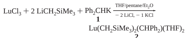
Figure 1. Molecular structure of [1(THF)_{0.5}]_\infty (30% probability thermal ellipsoids); hydrogen atoms (except H(1)) have been omitted for clarity. Selected bond lengths [Å] and angles [deg] (Cg is defined by the ring atoms C(8)–C(13)): K-C(1) 3.003(5), K-C(2) 3.248(4), K-C(8) 3.566(5), K-C(1'') 3.101(5), K-Cg' 3.067(3), K-C(11') 3.076(6), K-C(10') 3.140(5), K-C(12') 3.255(5), K-C(9') 3.437(5), K-C(13') 3.544(5), K-C(8') 3.698(5), K-O 2.778(4), C(1)-C(2) 1.441(7), C(1)-C(8) 1.429(8), C(1)-K-Cg' 111.17(11), K-C(1'')-K'' 165.4(2), C(1)-K-O 101.31(12), C(2)-C(1)-C(8) 132.1(5). Symmetry operations to generate equivalent atoms: (') 1.5-x, 0.5-y, z , (')' 1.25-x, -0.25+y, -0.25+z .
