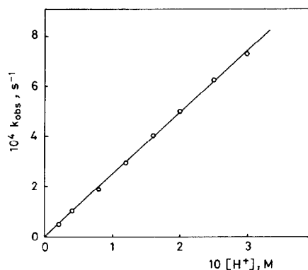
Fig. 2. Plot of k_{\text{obs}} vs. [\text{H}^+] at [\text{Cl}^-] = 0.1 M for the protonolysis of trans -[PtClMe(PET 3 ) 2 ] at 30 °C.
