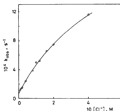
Fig. 3. Plot of k_{\text{obs}} vs. [\text{Cl}^-] at [\text{H}^+] = 0.2 M for the protonolysis of trans -[PtClMe(PET 3 ) 2 ] at 30 °C.
