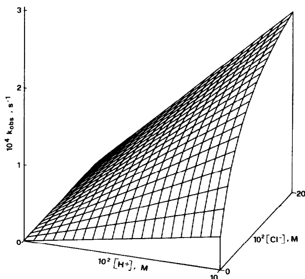
Fig. 4. 3-D representation of the dependence of k_{\text{obs}} on [\text{H}^+] and [\text{Cl}^-] for the protonolysis of cis -[PtPh 2 (PEtPh 2 ) 2 ] at 40 °C.
