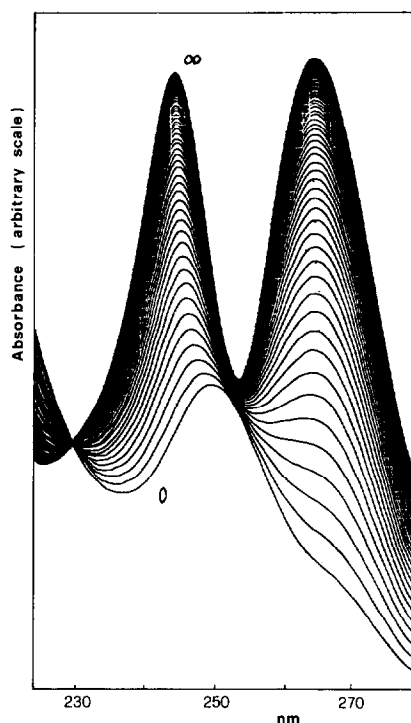
Fig. 1. Changes in optical density with time for the reaction \text{trans-[PtClMe(PEt}_3\text{)}_2\text{]} \xrightarrow[\text{H}^+, \text{Cl}^-]{\text{H}^+, \text{Cl}^-} \text{trans-[PtCl}_2\text{(PEt}_3\text{)}_2\text{]} + \text{CH}_4 at 30 °C.
