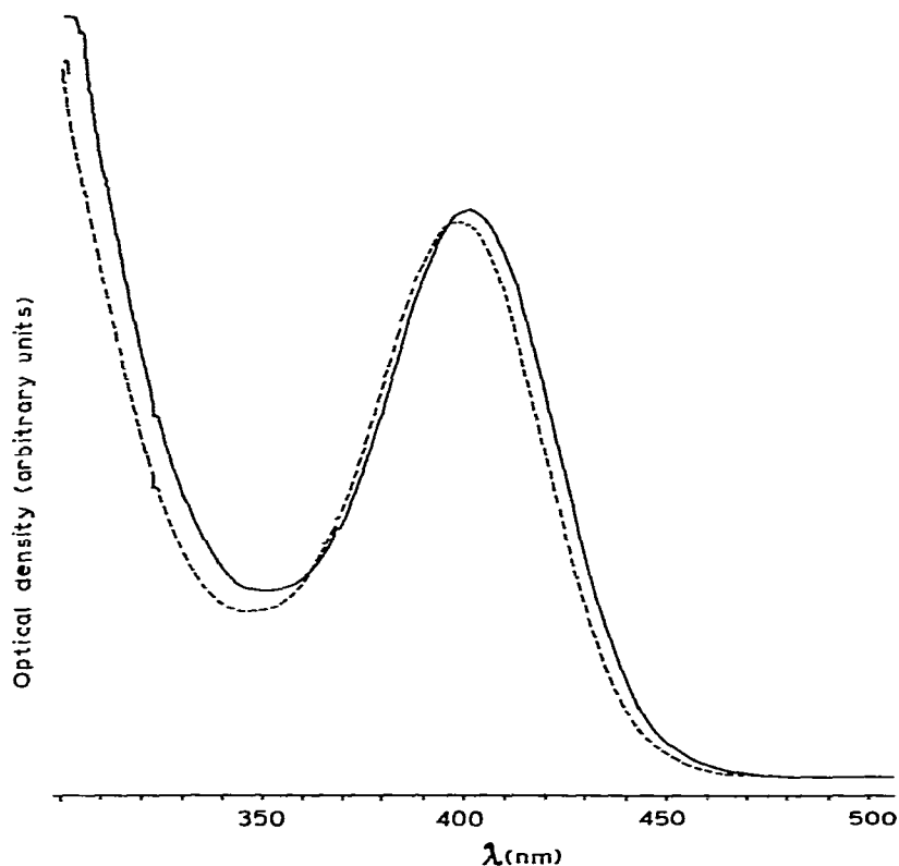
Fig. 2. The ultraviolet/visible spectrum of \text{Cr}(\text{CO})_5\text{Metz} in ethanol (---) and toluene (—).
