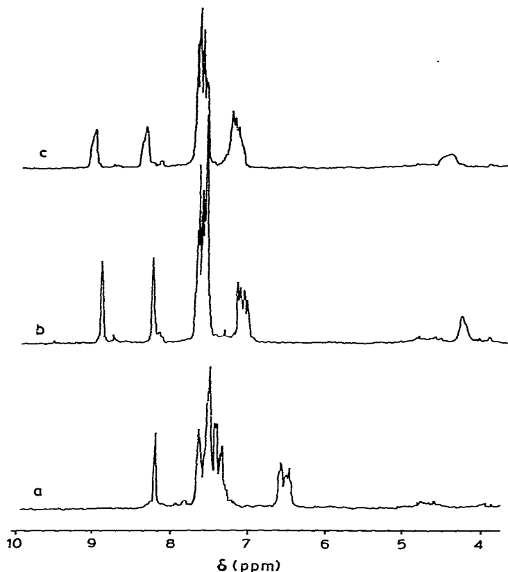
Fig. 4. The ^1\text{H} NMR spectrum of \text{W(CO)}_5\text{Phtzr} in (a) pure toluene- d_8 , (b) 20% (v/v) methanol- d_4 in toluene- d_8 , (c) 30% (v/v) methanol- d_4 in toluene- d_8 .
