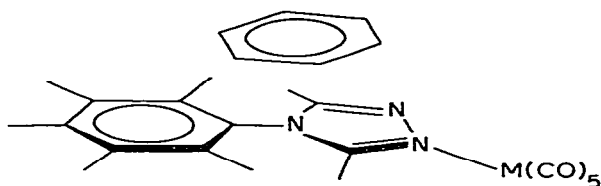
Fig. 5. Interaction of aromatic solvents with metal carbonyl triazole complexes.
