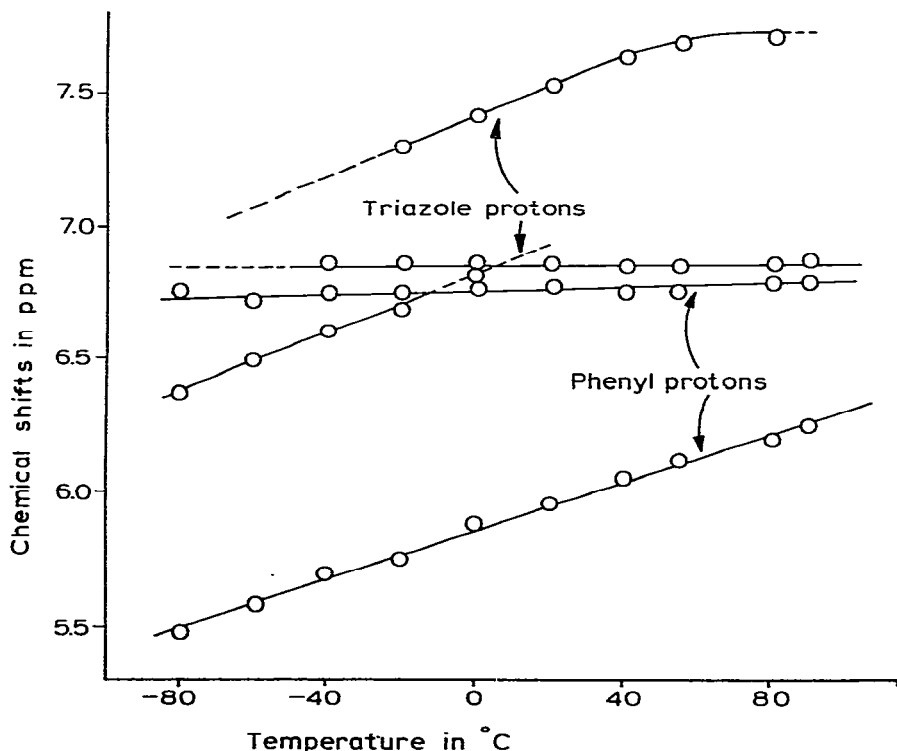
Fig. 6. Plot of the temperature dependence of the proton NMR spectrum of \text{W(CO)}_5\text{Phtrz} in \text{toluene-}d_8 . Solvent resonances occur between 7.0 and 7.1 ppm.
