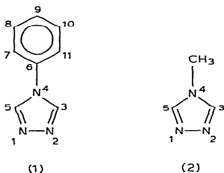
Fig. 1. Ligands: (1) 4-phenyl-1,2,4-triazole, (2) 4-methyl-1,2,4-triazole.
