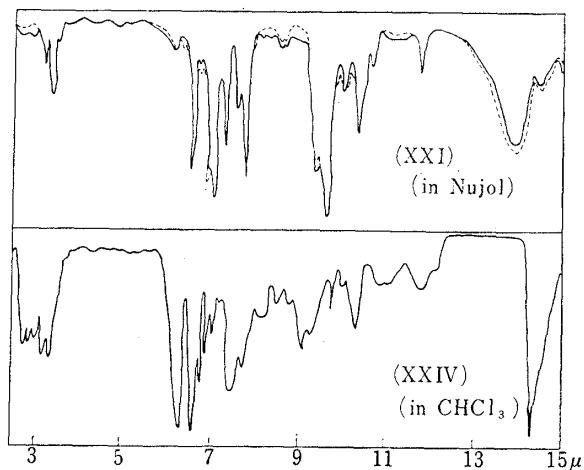
↓ Fig. 2. Infrared spectra — New synthesized compounds. ..... Authentic samples.
