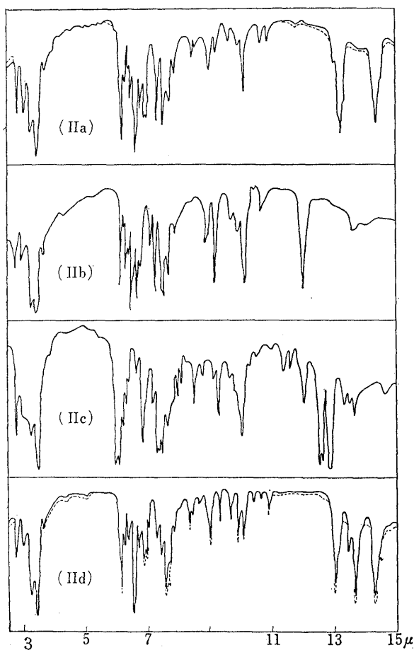
← Fig. 1. Infrared spectra of Thiazoles (in Nujol) — New synthesized compounds. ..... Authentic samples.
