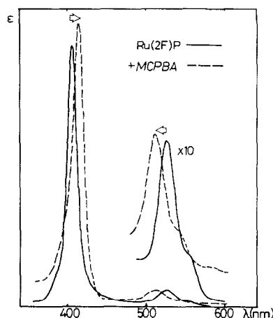
Fig. 3. Spectral changes of \text{Ru}_2\text{FP}(\text{CO})(\text{MeOH}) .
