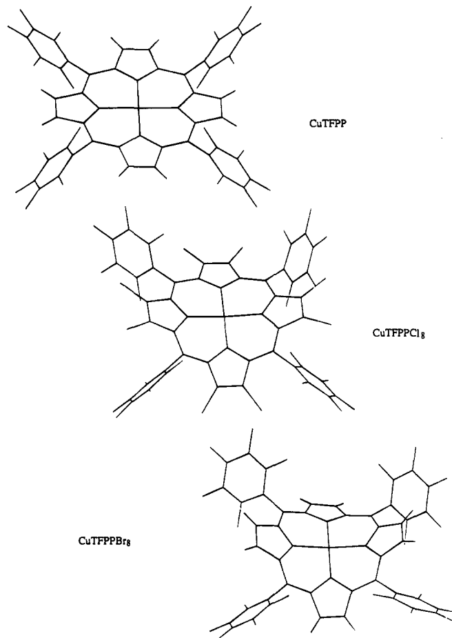
Figure 4. Molecular representations of the series CuTFPP, CuTFPPCl 8 , and CuTFPPBr 8 using the crystal structure coordinates. Both saddle and twist distortions increase in the octachloro and octabromo derivatives.
