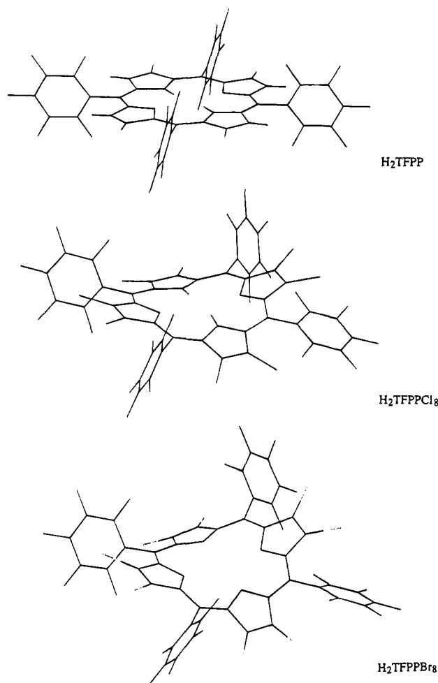
Figure 3. Molecular representations of the series H 2 TFPP, H 2 TFPPCl 8 , and H 2 TFPPBr 8 using the crystal structure coordinates. From the planar H 2 TFPP, the saddle distortion clearly increases upon further halogenation.
