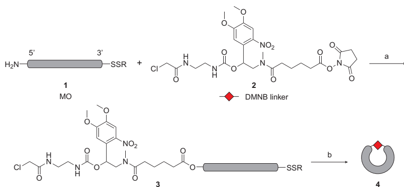
Fig. 2 Synthesis of cyclic cMOs. The DMNB linker is shown as an example. (a) 0.1 M Na 2 B 4 O 7 , pH 8.5, DMSO, 69–95%; (b) tris(2-carboxyethyl)phosphine, 0.1 M Tris-HCl buffer, pH 8.4, 84–92%. Adapted with permission from Yamazoe, S., Shestopalov, I. A., Provost, E., Leach, S. D., & Chen, J. K. (2012). Cyclic caged morpholinos: Conformationally gated probes of embryonic gene function. Angewandte Chemie, International Edition 51(28), 6908–6911.
