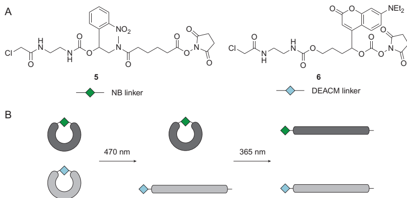
Fig. 3 Sequential and wavelength-activation of cyclic cMOs. (A) Chemical structures of the NB linker and the DEACM linker. (B) Concept of sequential activation of cMOs, prepared by using these two linkers. Adapted with permission from Yamazoe, S., Liu, Q., McQuade, L. E., Deiters, A., & Chen, J. K. (2014). Sequential gene silencing using wavelength-selective caged morpholino oligonucleotides. Angewandte Chemie, International Edition 53(38), 10114–10118.
