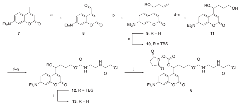
Fig. 4 Synthesis of the DEACM linker. (a) \text{SeO}_2 , dioxane, reflux, 42%; (b) allyltributyltin, \text{ZnCl}_2 , \text{CH}_3\text{CN}/\text{H}_2\text{O} , 83%; (c) TBSCl, imidazole, DMF, 97%; (d) \text{BH}_3\text{-Me}_2\text{S} , THF, 0^\circ\text{C} ; (e) \text{NaOH} , \text{H}_2\text{O}_2 , 0^\circ\text{C} —RT, 49% over two steps; (f) CDI, DCM; (g) ethylenediamine, DCM; (h) 2-chloroacetyl chloride, DIPEA, DCM, 0^\circ\text{C} —RT, 65% over three steps; (i) TBAF, THF, 0^\circ\text{C} , 44%; (j) DSC, DMAP, DCM, 82%. Adapted with permission from Yamazoe, S., Liu, Q., McQuade, L. E., Deiters, A., & Chen, J. K. (2014). Sequential gene silencing using wavelength-selective caged morpholino oligonucleotides. Angewandte Chemie, International Edition 53(38), 10114–10118.
