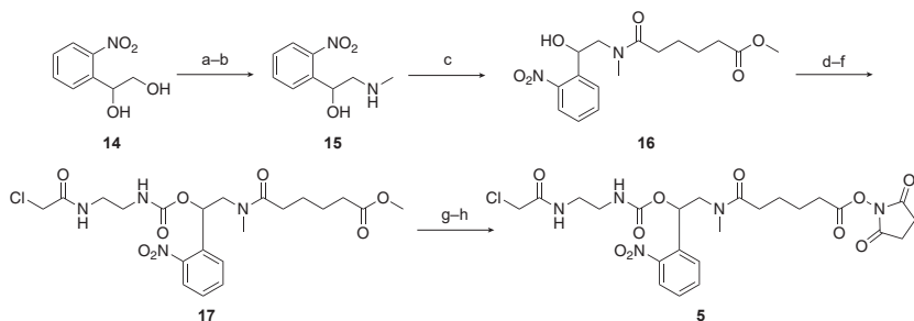
Fig. 5 Synthesis of the NB linker. (a) TsCl, pyridine, 99%; (b) methylamine, THF, 91%; (c) methyladipoyl chloride, DIPEA, \text{CH}_2\text{Cl}_2 , 41%; (d) CDI, \text{CH}_2\text{Cl}_2 ; (e) ethylenediamine, \text{CH}_2\text{Cl}_2 ; (f) 2-chloroacetyl chloride, \text{Et}_3\text{N} , \text{CH}_2\text{Cl}_2 , 65% over three steps; (g) LiOH, THF, \text{H}_2\text{O} ; (h) DSC, pyridine, \text{CH}_3\text{CN} , 62% over two steps. Ts = toluene-sulfonyl, DIPEA = N,N -diisopropylethylamine. Adapted with permission from Yamazoe, S., Liu, Q., McQuade, L. E., Deiters, A., & Chen, J. K. (2014). Sequential gene silencing using wavelength-selective caged morpholino oligonucleotides. Angewandte Chemie, International Edition 53(38), 10114–10118.
