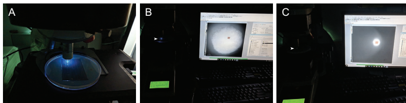
Fig. 6 Photoactivation of cMOs. (A) Irradiation set-up for zebrafish embryos using an agarose template in a Leica DM4500B upright fluorescence microscope equipped with a 20 \times , 0.5 NA water-immersion objective. (B) Global irradiation of an embryo controlled by Metamorph TM software. Full illumination of animal cells is shown. (C) Local irradiation of an embryo using similar set-up. Localized illumination of animal cells is shown. The illumination light beam has been indicated by the arrow-head.
