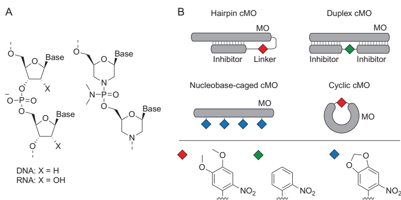
Fig. 1 Morpholinos and their caged versions. (A) DNA/RNA and MO chemical structures. (B) cMO design strategies showing hairpin, duplex, nucleobase-caged, and cyclic cMOs. The photolabile moiety has been indicated as diamond shapes. Adapted with permission from Yamazoe, S., Shestopalov, I. A., Provost, E., Leach, S. D., & Chen, J. K. (2012). Cyclic caged morpholinos: Conformationally gated probes of embryonic gene function. Angewandte Chemie, International Edition 51(28), 6908–6911.
