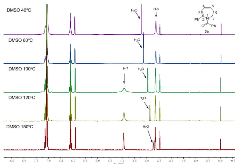
Figure 7. Variable temperature 1 H NMR spectra of 3a . The signals at ca. 2.5 are protons of DMSO.
