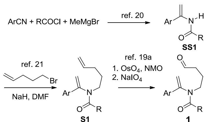
Figure 2. Preparation of substrates 1 .
