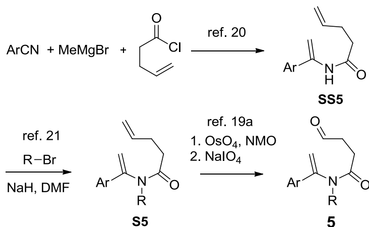
Figure 4. Preparation of substrates 5 .
