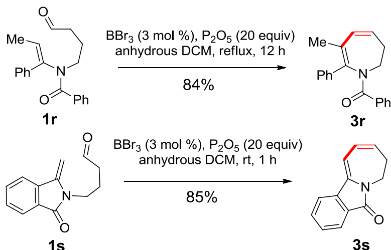
Figure 3. Synthesis of 3r and 3s .
