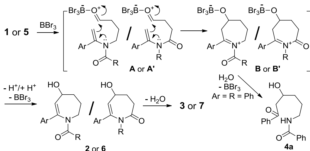
Figure 9. Plausible reaction mechanism.
