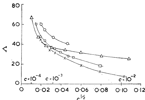
FIGURE 1. Conductance \Lambda (cm. 2 ohm -1 mole -1 ) of \text{NbCl}_5 , Diarsine and \text{TaCl}_5 , Diarsine in nitromethane as function of concentration
