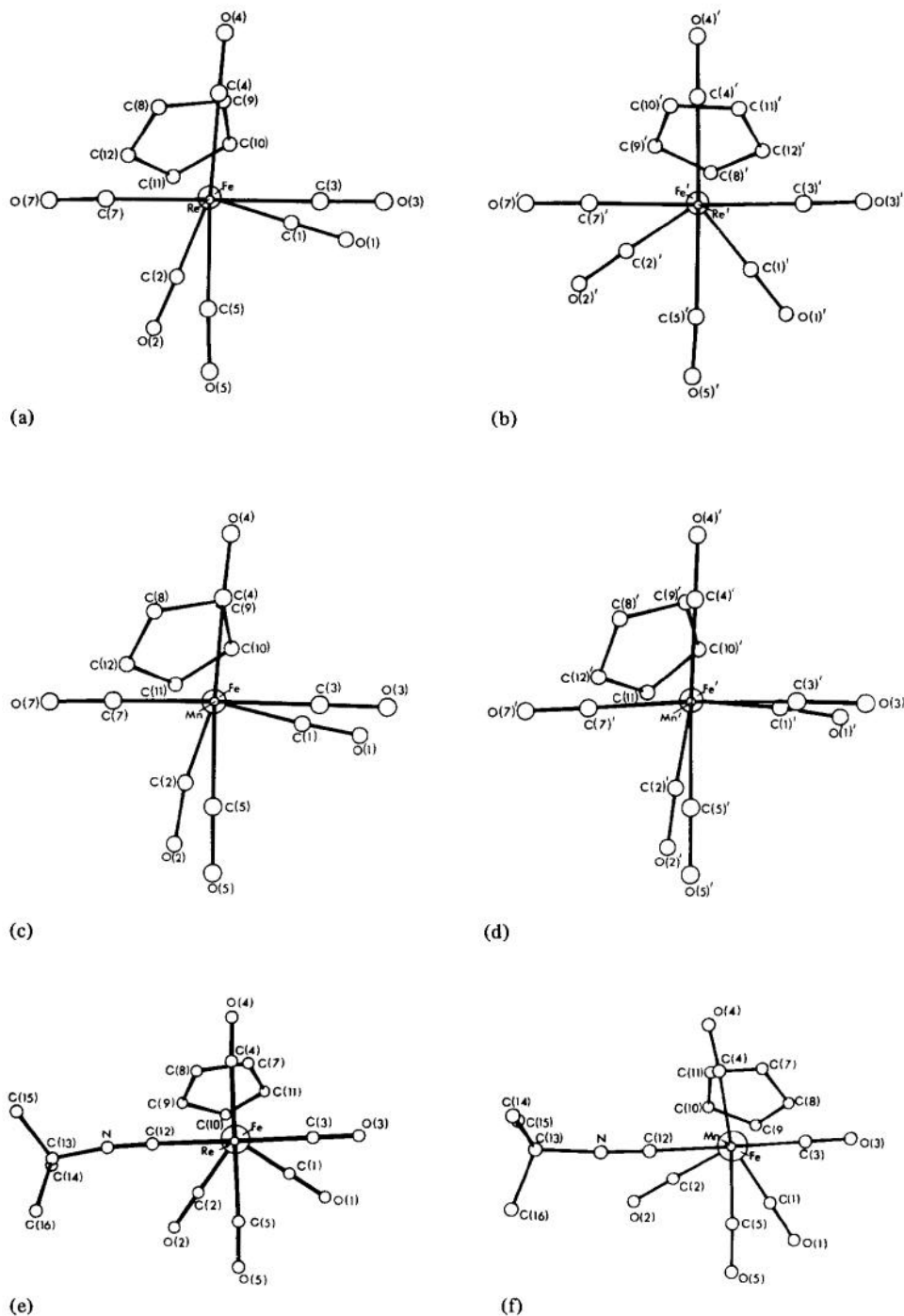
Fig. 2. Newman projections of structures 1–4 viewed down the metal–metal bond. (a) and (b) [(\eta^5\text{-C}_5\text{H}_5)\text{Fe}(\text{CO})_2\text{Re}(\text{CO})_5] (1); (c) and (d) [(\eta^5\text{-C}_5\text{H}_5)\text{Fe}(\text{CO})_2\text{Mn}(\text{CO})_5] (2); (e) [(\eta^5\text{-C}_5\text{H}_5)\text{Fe}(\text{CO})_2\text{Re}(\text{CO})_4(\text{CNBu-t})] (4); (f) [(\eta^5\text{-C}_5\text{H}_5)\text{Fe}(\text{CO})_2\text{Mn}(\text{CO})_4(\text{CNBu-t})] (3).
