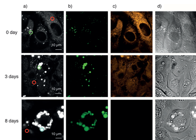
Figure 3. Confocal microphotographs of 3T3L1 preadipocytes (top) and adipocytes after 3 days (middle) and 8 days (bottom) of differentiation. The cells were stained with 1 for 2 h prior to examination: a) Lambda stack images in the emission range from \lambda = 416 to 689 nm with excitation at 405 nm. b, c) Linear-deconvolution images using reference spectra of selected pixels. The exhibited emission maxima in the range of \lambda = 521 –530 nm (green circle) and \lambda = 556 –565 nm (red circle), are shown in green and orange, respectively. d) Bright-field images.
