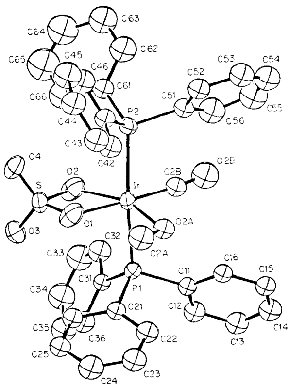
Fig. 1. Labelling of atoms in the deconvoluted molecular structure of disordered \text{Ir}(\text{OMe})(\text{CO})\text{-(PPh}_3)_2(\text{SO}_4) .
