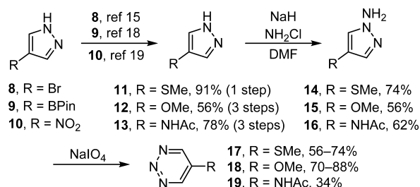
Scheme 1. Synthesis of 1,2,3-Triazines 17–19
