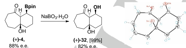
Scheme 6. Stereospecific C-B bond oxidation of (+)-4.
