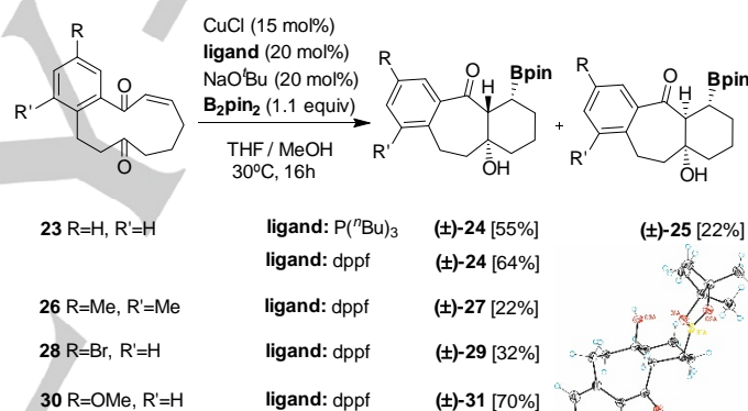
Scheme 4. Cu-catalyzed diastereoselective borylative transannular reaction on cycloundecane substrates.
