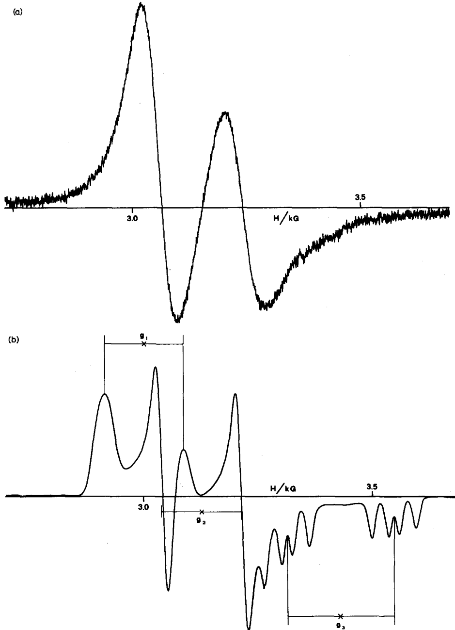
Fig. 3. ESR spectrum of [\text{Ir}(\text{C}_6\text{H}_5)(\text{CO})(\text{PPh}_3)_3]^+ 1.0 mM in DCE 0.2 M TBAP, 0.1 M \text{PPh}_3 at 298 K (a) and 120 K (b).
