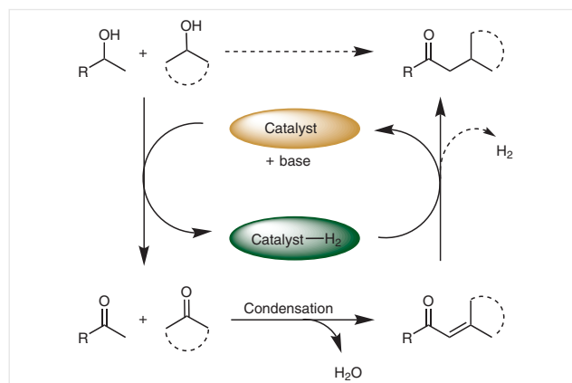
Scheme 1 Borrowing-hydrogen methodology in cross-coupling of secondary alcohols
