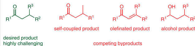
Scheme 3 Ruthenium-catalyzed direct cross-coupling of secondary alcohols and selectivity challenges. (Reprinted with permission from reference 12. © 2019, American Chemical Society)
