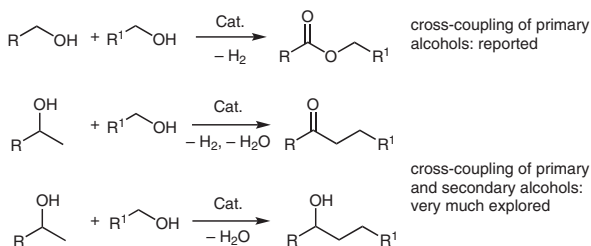
Scheme 2 Catalytic self-couplings and cross-couplings of alcohols. (Reprinted with permission from reference 12. © 2019, American Chemical Society.)
