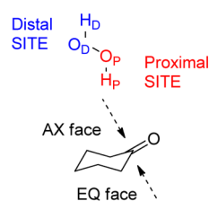
Scheme 3. Different Modes of Approach to the Cyclohexanone Molecule Considered in the Present Study and the Labeling Adopted for the Hydrogen Peroxide Molecule
