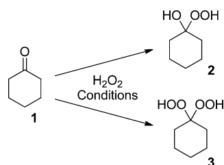
Scheme 2. Process Investigated in the Present Work
