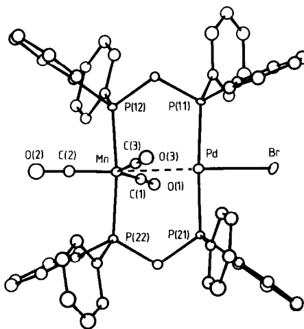
Fig. 1. Molecular structure of \text{MnPd}(\text{CO})_3(\text{dppm})_2\text{Br} (2). Selected bond lengths ( \text{\AA} ) and angles are: \text{Pd}\cdots\text{Mn} 2.810(2), \text{Pd}-\text{Br} 2.547(2), \text{Pd}-\text{P}(11) 2.299(4), \text{Pd}-\text{P}(21) 2.290(4), \text{Mn}-\text{P}(12) 2.254(3), \text{Mn}-\text{P}(22) 2.276(3), \text{Mn}-\text{C}(1) 1.96(1), \text{Pd}\cdots\text{C}(1) 2.44(1), \text{Pd}\cdots\text{O}(1) 3.00(1), \text{Mn}-\text{C}(2) 1.63(2), \text{Mn}-\text{C}(3) 1.78(1), \text{Pd}\cdots\text{C}(3) 2.95(1), \text{Mn}-\text{C}(1)-\text{O}(1) 174(1)^\circ , \text{Mn}-\text{C}(3)-\text{O}(3) 175(1)^\circ .
