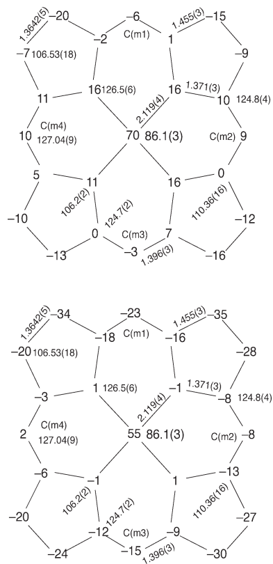
Figure 7. Mean-plane diagrams for anion 1 of [\text{Na}(222)][\text{Fe}(\text{OEP})(\text{SH})] \cdot 0.5\text{C}_6\text{H}_6 . The values of the atomic displacements from 24-atom (top) and 4-nitrogen-atom (bottom) mean planes are given in units of 0.01 Å. Also entered on the diagrams are mean porphyrin core bond lengths in angstroms and mean bond angles in degrees.
