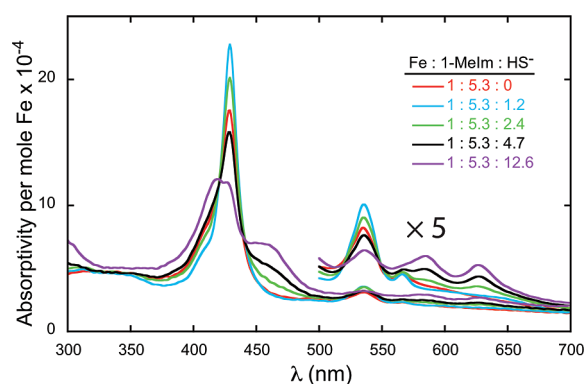
Figure 5. UV-vis molar absorptivity plots of chlorobenzene solutions of [Fe(TMP)] with varied Fe/1-Melm/HS − ratios. The concentration of [Fe(TMP)] ranged from 0.069 to 0.053 mM, while 1-Melm ranged from 0.36 to 0.28 mM and HS − was adjusted according to the ratios reported in the figure. The decrease in the [Fe(TMP)] concentration is due to dilution incurred upon ligand addition. From 500 to 700 nm, plots are shown at both regular scale and magnified 5 \times .
