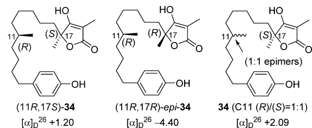
Figure 2. Diastereomers of 34 and their [\alpha]_D measured at c = 0.61 in MeOH. For the synthesis of epi - 34 and C-11 racemic 34 (which showed the contribution of each stereogenic center to the observed optical rotation); see the Supporting Information.
