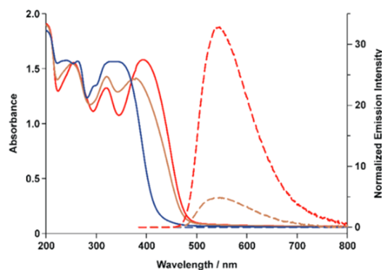
Figure 2. Absorption spectra (solid lines, left scale) and emission spectra (dashed lines, right scale; \lambda_{\text{ex}} = 380 nm) of a drop-casted film of 1 . The red lines are of 1-Z, the blue lines correspond to PSS 450 (>90% 1-E), and the brown lines depict the bands at PSS 360 .
