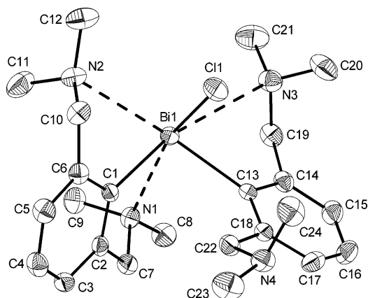
Figure 7. Molecular structure of the ( R_{N1}, S_{N2} )( S_{N3} ) isomer of 5 (ORTEP drawing with 30% probability ellipsoids) with the labeling scheme for the atom positions. Hydrogen atoms have been omitted for clarity.
