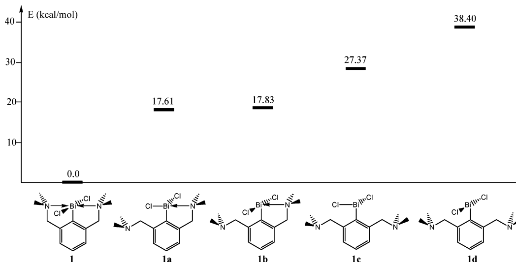
Figure 5. Calculated relative energies of different isomers of [2,6-(\text{Me}_2\text{NCH}_2)_2\text{C}_6\text{H}_3]\text{BiCl}_2 , 1 .
