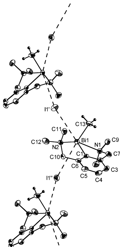
Figure 6. Part of the polymeric chain of 4 (ORTEP drawing with 30% probability ellipsoids) with the labeling scheme for the atom positions [symmetry equivalent atoms ( 1-x , -0.5+y , 1.5-z ) and ( 0.5+x , y , 1.5-z ) for I1' and I1'' , respectively]. Hydrogen atoms, less those of the methyl group attached to the metal, have been omitted for clarity.
