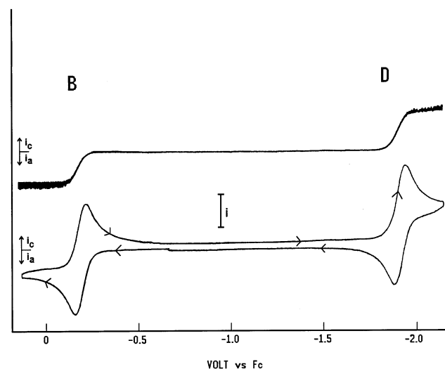
Fig. 1. Voltammetry of 0.5 mM 1 in \text{CH}_2\text{Cl}_2/0.1 \text{ M } [\text{Bu}_4\text{N}][\text{PF}_6] at 228 K at Pt electrodes. Top, rotating Pt electrode scan, \nu = 2 \text{ mV s}^{-1} ; bottom, CV scan, \nu = 0.20 \text{ V s}^{-1} , at twice the current sensitivity. Waves B and D refer to the labels from text, processes \mathbf{1}^+/\mathbf{1}^{2+} and \mathbf{1}^+/\mathbf{1} , respectively.
