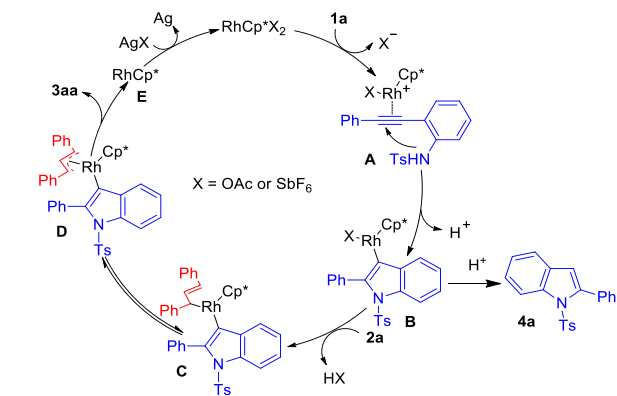
Scheme 6. Plausible Mechanism
