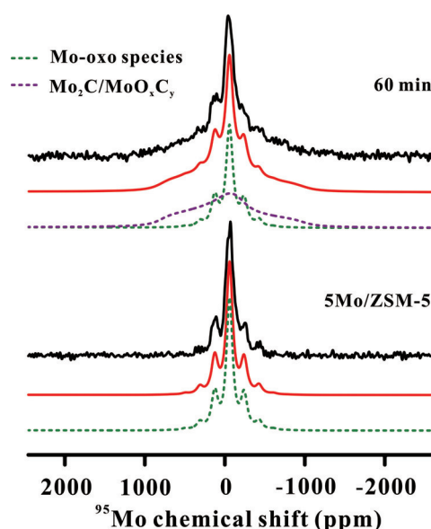
Figure 2. Experimental and deconvoluted ^{95}\text{Mo} WURST-QCPMG MAS NMR spectra (acquired at 35.2 T) of fresh 5Mo/ZSM-5 and 5Mo/ZSM-5 reacted for 60 min at 973 K. Solid (black —): experimental, solid (red —): simulated, dash (purple —, green —): deconvoluted.
