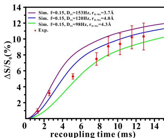
Figure 4. Experimental ^1\text{H}\{^{95}\text{Mo}\} S-RESPDOR dephasing fraction of Brønsted acidic protons in 5Mo/ZSM-5 as a function of recoupling time. The best fit of the experimental results was determined to be f=0.15 and D_{IS}=120 Hz, corresponding to a ^1\text{H} - ^{95}\text{Mo} internuclear distance of 4.0 Å. f denotes the pre-factor parameter and D_{IS} is the heteronuclear dipolar interaction between two spins used in the analytical formula. Sim. and exp. represent simulated and experimental curves, respectively.
