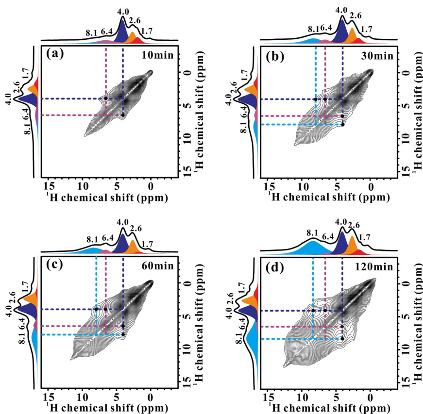
Figure 5. 2D ^1\text{H} - ^1\text{H} spin diffusion NMR spectra (acquired at 9.4 T) of 5Mo/ZSM-5 reacted at 973 K for a) 10 min, b) 30 min, c) 60 min, and d) 120 min. Mixing time is 300 ms.
