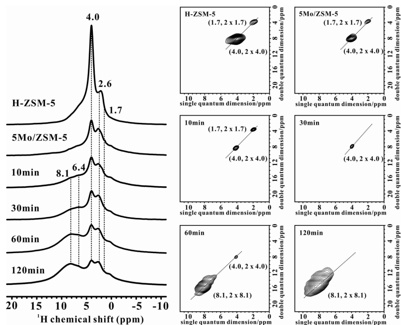
Figure 1. ^1\text{H} MAS NMR (left) and ^1\text{H} - ^1\text{H} DQ-SQ (right) MAS NMR spectra (acquired at 9.4 T) of H-ZSM-5, fresh 5Mo/ZSM-5 and reacted 5Mo/ZSM-5 samples for 10–120 min at 973 K.
