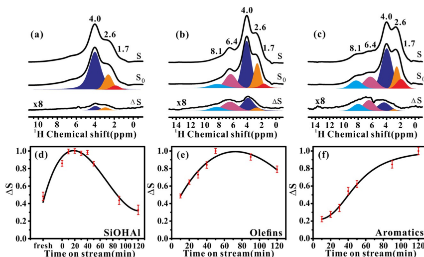
Figure 3. a)–c) ^1\text{H}\{^{95}\text{Mo}\} S-RESPDOR NMR spectra (acquired at 18.8 T) of a) fresh 5Mo/ZSM-5, b) 5Mo/ZSM-5 reacted for 30 min and c) for 120 min of MDA reaction at 973 K. Recoupling time is 5.12 ms. d)–f) Normalized \Delta S of d) Brønsted acid, e) olefins, and f) aromatics versus MDA reaction time. \Delta S = S_0 - S .
