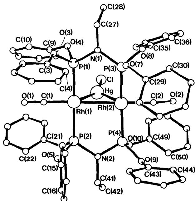
Fig. 1. The molecular structure of [\text{Rh}_2\text{HgCl}(\mu_2\text{-H})(\text{CO})_2\{\mu\text{-(PhO)}_2\text{PN(Et)P(OPh)}_2\}_2] (with omission of the \mu\text{-H} ). Some relevant interatomic distances and angles: Rh(1)—Rh(2), 2.762(1) ; Rh(1)—Hg, 2.711(1) ; Rh(2)—Hg, 2.778(1) ; Rh(1)—P(1), 2.253(2) ; Rh(1)—P(2), 2.254(2) ; Rh(2)—P(3), 2.242(2) ; Rh(2)—P(4), 2.257(2) ; Hg—Cl, 2.470(3) Å; Rh(1)—Hg—Rh(2), 60.4(0) ; Rh(1)—Rh(2)—Hg, 58.6(0) ; Rh(2)—Rh(1)—Hg, 61.0(0) ; P(1)—Rh(1)—Rh(2), 91.1(1) ; P(2)—Rh(1)—Rh(2), 91.2(1) ; P(3)—Rh(2)—Rh(1), 90.1(1) ; P(4)—Rh(2)—Rh(1), 91.4(1) ; Rh(1)—Rh(2)—C(2), 173.3(4) ; Rh(2)—Rh(1)—C(1), 173.3(4) ; Rh(1)—Hg—Cl, 153.3(1) ; Rh(2)—Hg—Cl, 145.4(1) ; P(1)—N(1)—P(3), 117.9(4) ; P(2)—N(2)—P(4), 118.7(4)^\circ .
