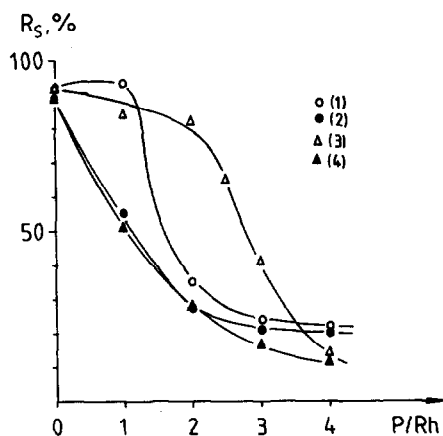
Fig. 1. Influence of the phosphine/Rh ratio on the regioselectivity of hydroformylation; reaction conditions: 100 °C, 15 bar ( \text{CO}/\text{H}_2 = 1/1 ); \text{Rh}/\text{N}/\text{MMA} = 1/15/20 ; 3 h. (1) [\text{Rh}(\text{NBD})\text{Cl}]_2 + \text{PPh}_3 , (2) [\text{Rh}(\text{NBD})\text{Cl}]_2 + \text{PPh}_3 + \text{Et}_3\text{N} , (3) [\text{Rh}(\text{NBD})\text{Cl}]_2 + \text{PBu}_3 , (4) [\text{Rh}(\text{NBD})\text{Cl}]_2 + \text{PBu}_3 + \text{Et}_3\text{N} .
