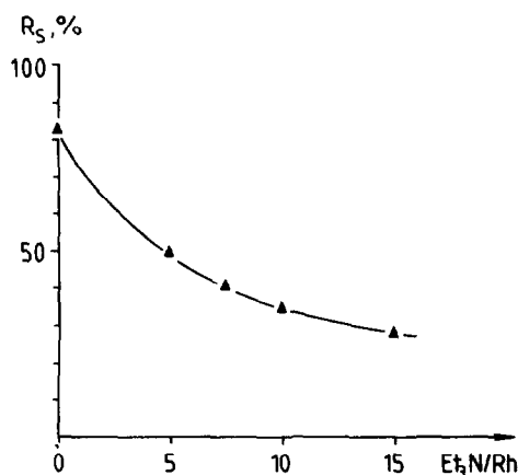
Fig. 2. Influence of the \text{Et}_3\text{N}/\text{Rh} ratio on the regioselectivity of hydroformylation; reaction conditions: 100 °C, 15 bar ( \text{CO}/\text{H}_2 = 1/1 ); 3 h; \text{Rh}/\text{PBu}_3/\text{MMA} = 1/2/20 .
