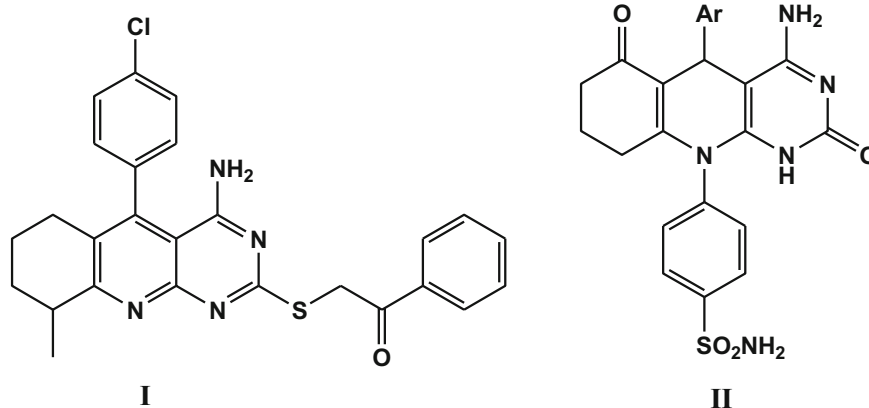
Fig. 2 Structure of potent anticancer tetrahydropyrimidoquinolines
