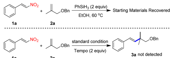
Scheme 3. Control Experiments
