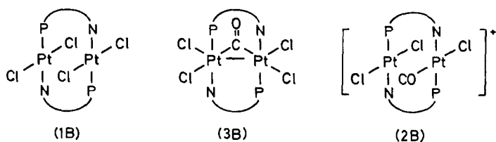
Fig. 1. Possible structures of compounds 1, 2 and 3.
