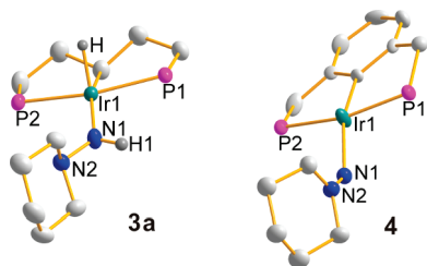
Figure 2. ORTEP diagrams of (D'BPP)Ir(H)(NHNC 5 H 10 ) ( 3a , left, Ir–N = 1.9875(18) Å, N–N = 1.435(2) Å, <H–Ir–C = 73.9(8)°, <C–Ir–N = 154.47(9)°, <Ir–N–N = 132.53(14)°, <N–N–C = 108.83(17)° and 108.61(17)°, <C–N–C = 109.37(17)°) and (PCP)Ir(H)(NHNC 5 H 10 ) ( 4 , right, Ir–N = 2.008(11) Å, N–N = 1.244(16) Å, <C–Ir–N = 154.9(4)°, <Ir–N–N = 135.1(12)°, <N–N–C = 128.4(16)° and 118.8(15)°, <C–N–C = 112.8(14)°) ( tert -butyl groups and most H atoms omitted for clarity).
