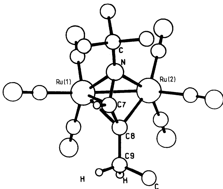
Fig. 10. Structure of \text{Ru}_2(\text{CO})_6(1\text{-t-Bu-N}\equiv\text{C(H)}\equiv\text{CCH}_2\text{CH}_3) .
