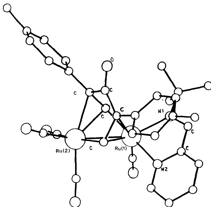
Fig. 7. Structure of \text{Ru}_2(\text{CO})_4\{((t\text{-Bu-Pyca})(\text{HC}\equiv\text{CR})_2(\text{CO}))\} .
