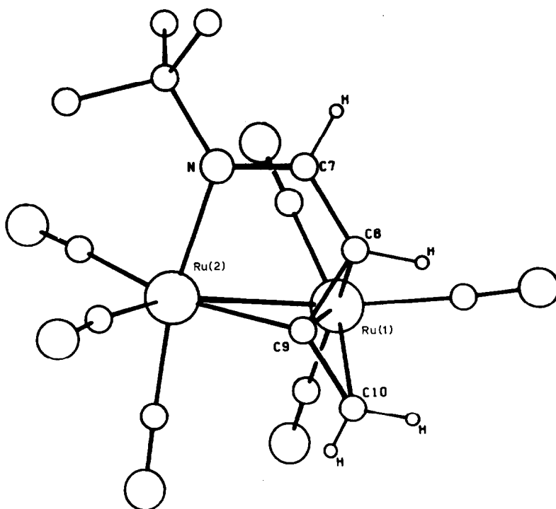
Fig. 11. Structure of \text{Ru}_2(\text{CO})_6(1\text{-t-Bu-N}=\text{C(H)}(\text{H})\text{C}=\text{C}=\text{CH}_2) .
