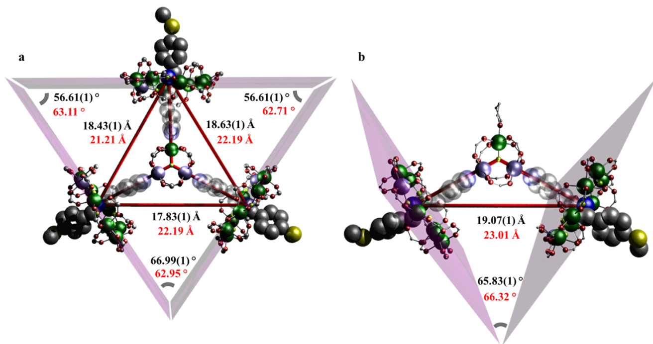
Figure 1. The structures of 3 and 4 in the crystal, with select metric parameters indicated (black, XRD; red, AMDS). (a) 3 showing angles between the mean planes of the \{\text{Cr}_7\text{Ni}\} rings, and the distances between N atoms of secondary ammonium groups; (b) 4 showing angles between the mean planes of the \{\text{Cr}_7\text{Ni}\} rings and the distances between N atoms of secondary ammonium groups. Colors: Cr, green; Ni, purple; O, red; F, yellow; N, blue; C, silver; S, dull yellow. H-atoms and methyl groups of pivalates excluded for clarity.
