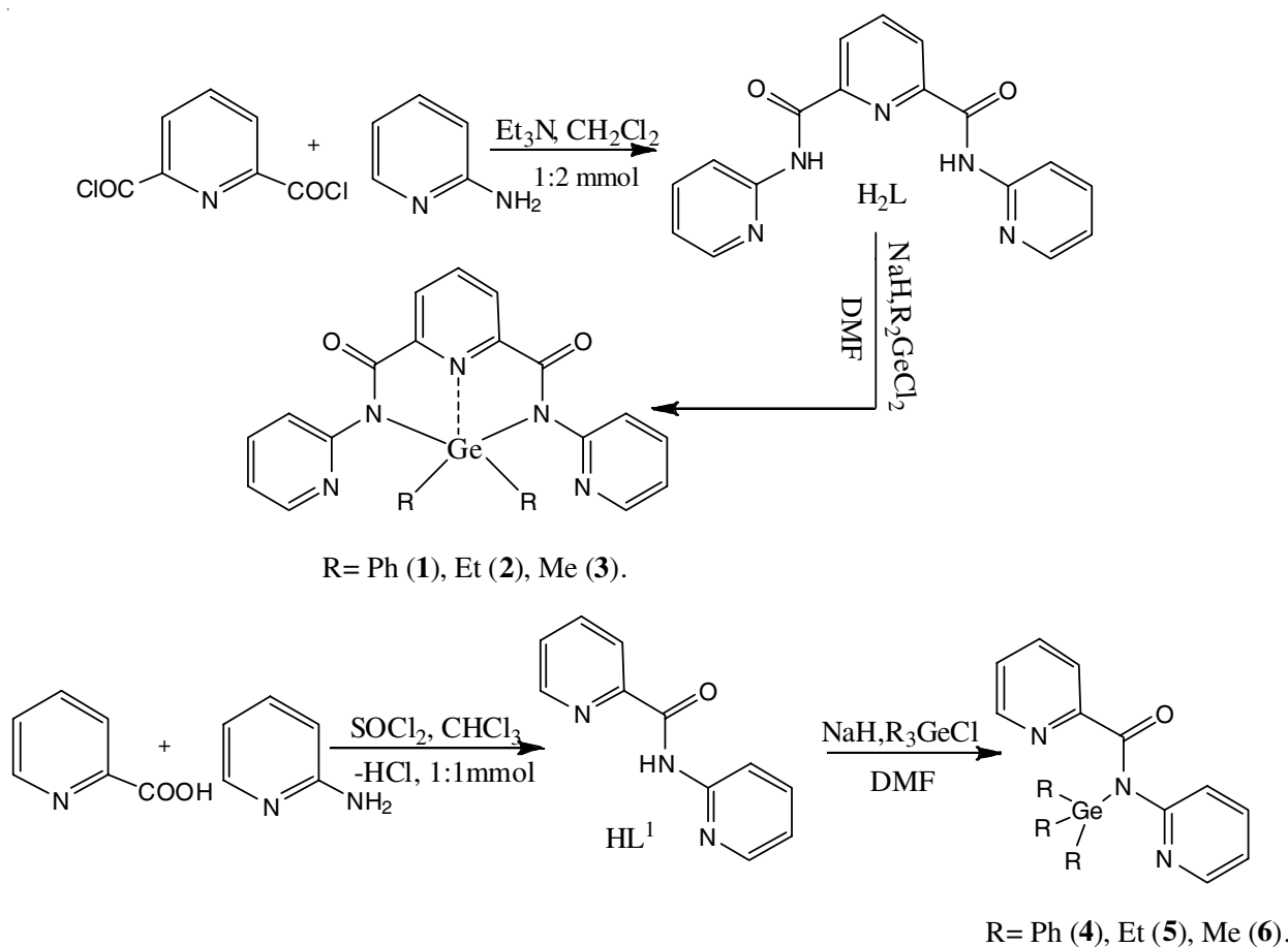
Scheme-I: Preparation of germanium complexes
