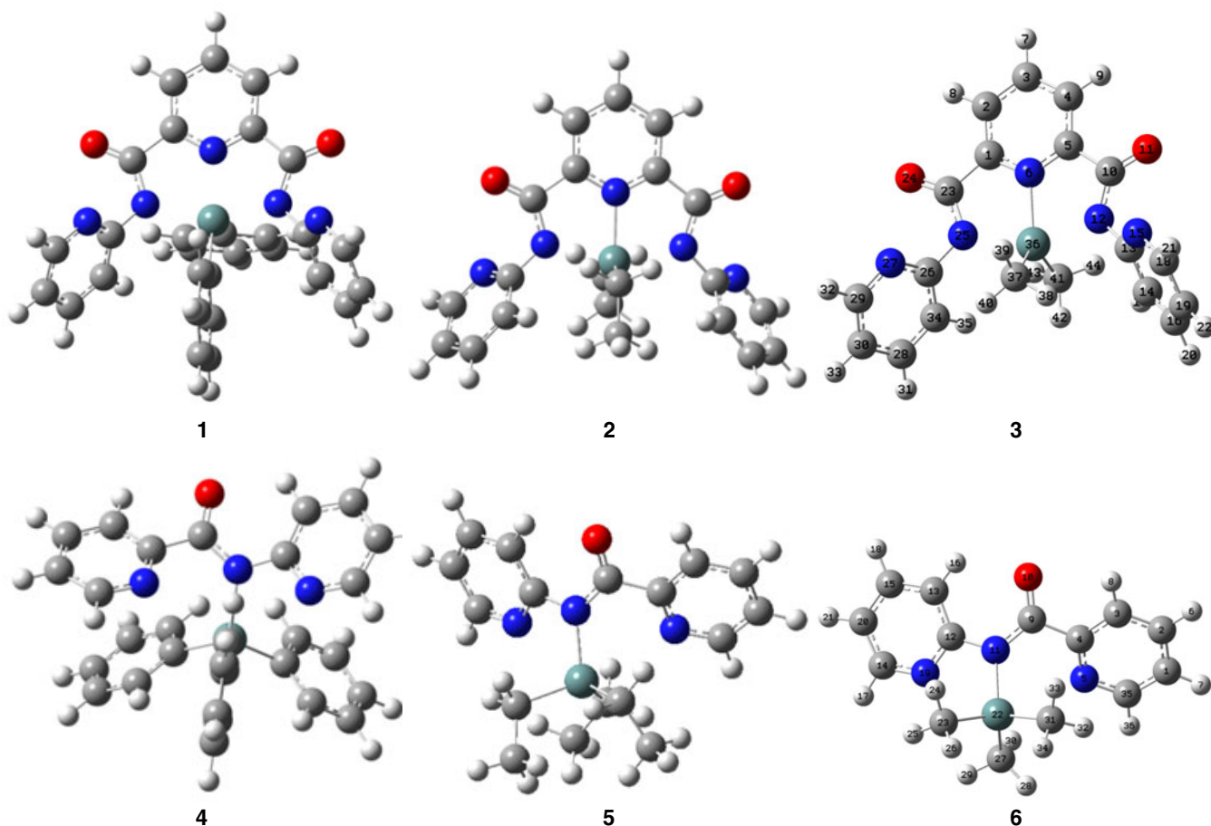
Fig. 2. Optimized structure of germanium complexes 1–6
