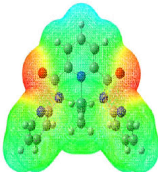
Fig. 3. MESP plot and NPA charges of respective atoms for H 2 L and complex 3
