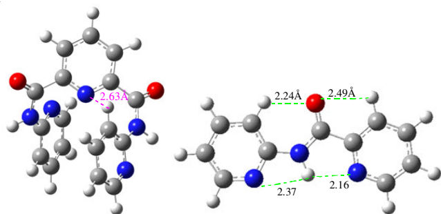
Fig. 1. Optimized structure of ligands H_2L and HL^1
