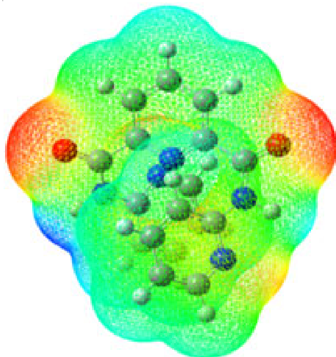
Fig. 3. MESP plot and NPA charges of respective atoms for H 2 L and complex 3
