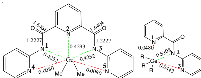
Fig. 4. Wiberg bond index analysis
