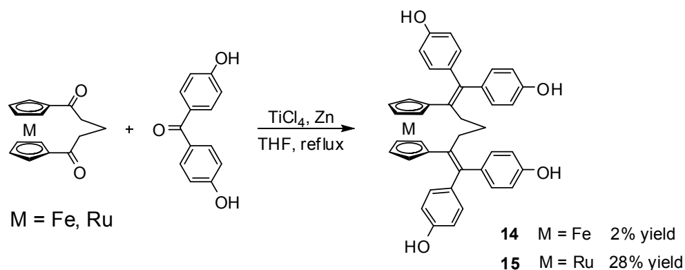
Scheme 3. Synthesis of tetraphenols 14 and 15 .
