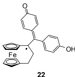
Chart 2. Major reactive intermediate for 1b . 62
