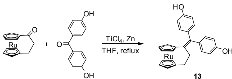
Scheme 2. Synthesis of ruthenocenophane 13 .
