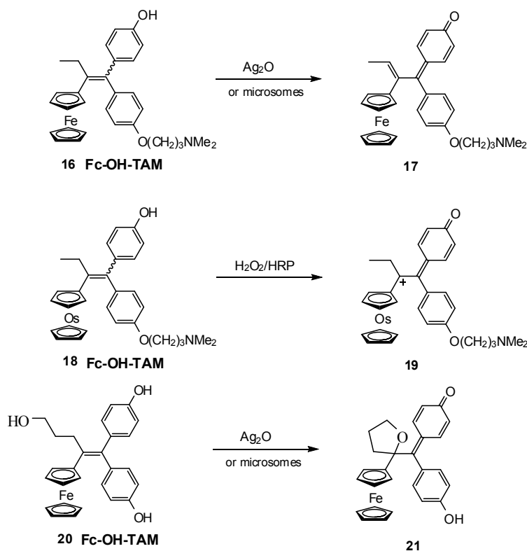
Scheme 4. Oxidation of 16 , 18 and 20 .
