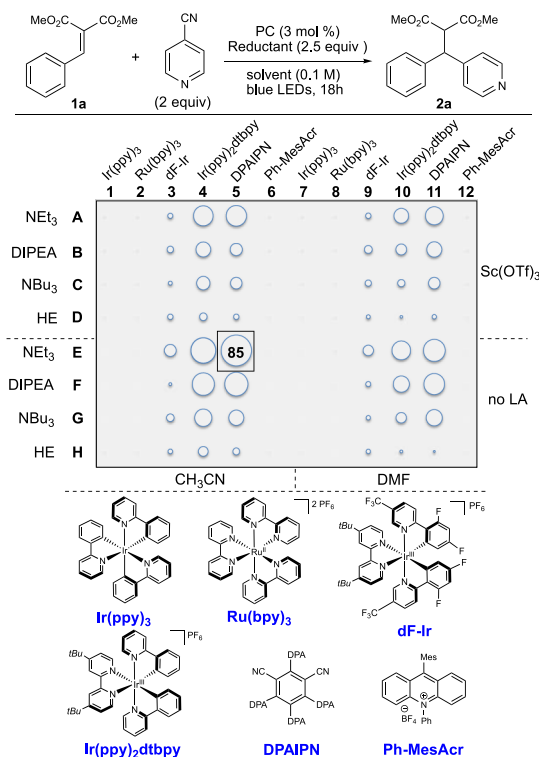
Scheme 1. Reaction Optimization Using HTE a
