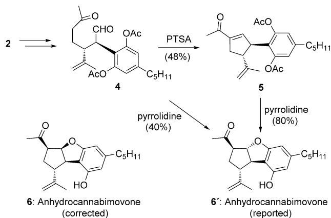
Scheme 1. Synthesis of anhydrocannabimovone ( 6 ) from cannabidiol (CBD, 2 ). [9]
