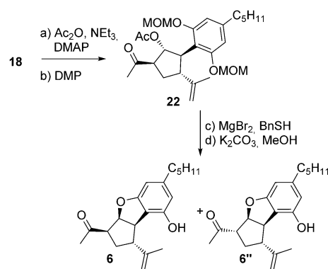
Scheme 6. a) Ac 2 O, Et 3 N, DMAP, CH 2 Cl 2 , −30°C, 1 h, 50% (56% brsm); b) DMP, NaHCO 3 , CH 2 Cl 2 , 25°C, 1 h, 73%; c) MgBr 2 , BnSH, Et 2 O, 25°C, 24 h, 82%; d) K 2 CO 3 , MeOH, 25°C, 15 min, 60% ( 6 ) and 19% ( 6'' ).
