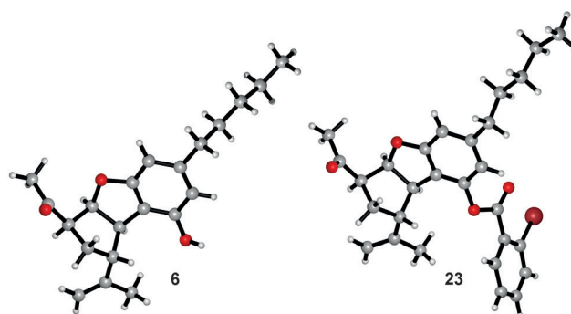
Figure 2. X-Ray structures for 6 and 23 .
