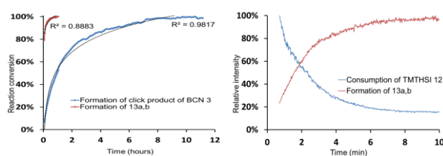
Figure 2. Determination of the reaction rate of the strain-promoted azide-alkyne cycloaddition reaction of TMTHSI 12 and benzyl azide by NMR (left) and IMS - MS (right). Reaction of 5 mM TMTHSI and 6.38 mM benzyl azide (1:1.3) in CDCl 3 at 25 °C as compared to the reaction of endo-BCN-OH 3 (4.75 mM) and benzyl azide (6.02 mM) determined by NMR in CDCl 3 (left). Reaction rate of 5mM TMTHSI and benzyl azide (1:1) in water/acetonitrile (1:3) and 0.01% acetic acid at 25 °C by MS (right). The relative intensity of TMTHSI 12 consumption and triazole product 13a,b formation is shown (for more details see Electronic Supplementary Information).
