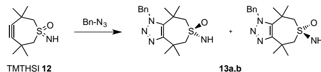
Scheme 2. Strain promoted azide-alkyne cycloaddition of prochiral TMTHSI 12 and benzyl azide to furnish enantiomeric triazole adducts 13a and 13b , in which merely the stereochemistry of the sulfur atoms was indicated.
