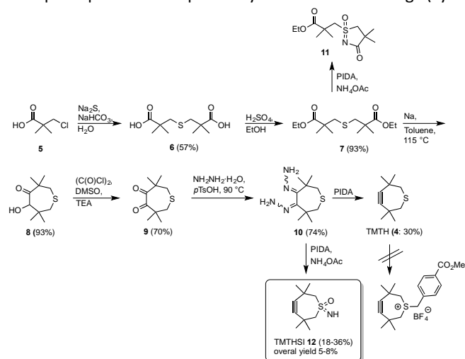
Scheme 1. Synthesis of TMTH 4 . [13,14,15,17] attempted alkylation of TMTH, preparation of sulfoximine and its subsequent cyclization to 11 using PIDA and synthesis of TMTHSI 12 .
