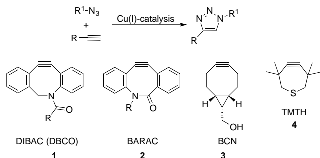
Figure 1. The classic Cu(I) catalyzed 'click' reaction and the most important examples of reagents for strain-promoted azide-alkyne cycloaddition reactions.
