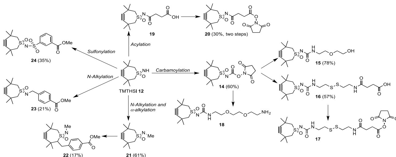
Scheme 3. Functionalization of TMTHSI 12 followed introduction by linkage moieties for introduction of for example API's.
