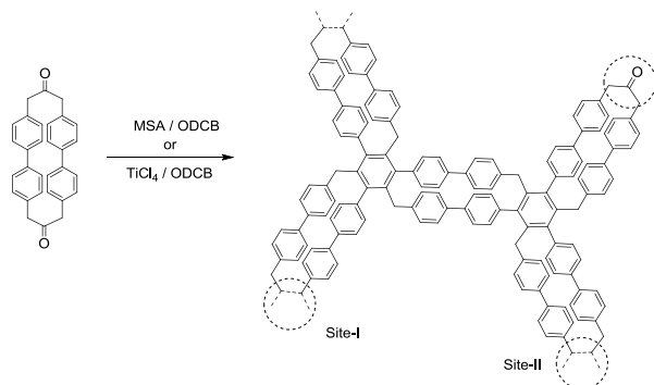
Scheme 2. Synthesis of microporous polymer network through acid catalyzed cyclotrimerization of macrocycle MC and idealized structure of the resulting crosslinked polymer network.
