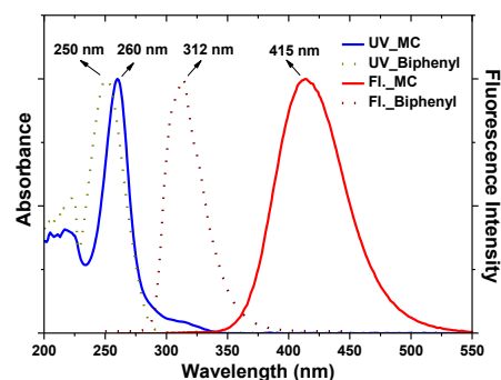
Fig. 2 Normalized UV-vis and fluorescence spectra of the macrocycle MC and biphenyl (as a comparison) recorded in dichloromethane ( \lambda_{\text{ext}} : 245 nm for MC and 235 nm for biphenyl).
