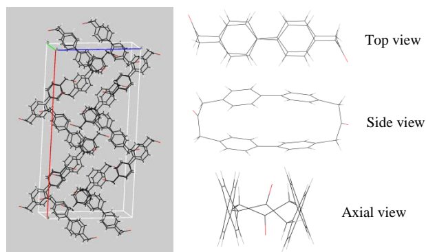
Fig. 1 Single crystal X-ray structure of the macrocycle MC including the geometry of the single molecules and packing in the unit cell.
