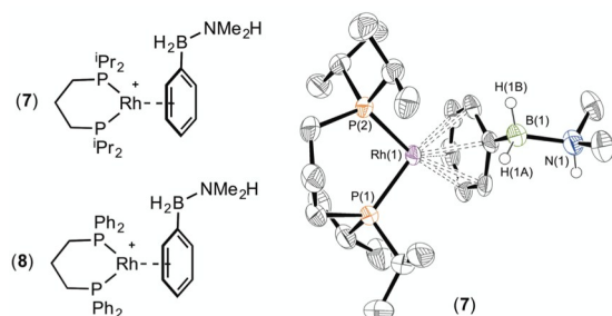
Figure 3: X-ray molecular structure of (7). [\text{BARF}_4]^- anion and selected H atoms omitted for clarity. Ellipsoids shown at 50% probability level. Selected bond lengths (Å) and angles (°): Rh(1)–P(1) 2.2441(11), Rh(1)–P(2) 2.2422(10), Rh(1)–Ph Centroid 1.851, B(1)–N(1) 1.618(6); P(1)–Rh(1)–P(2) 94.27(4).
