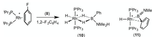
Scheme 7: Complexes 10 and 11. [\text{BARF}_4]^- anions not shown.
