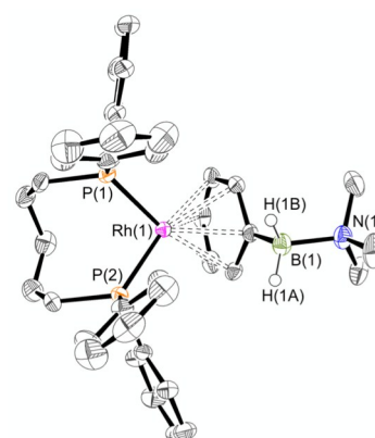
Figure 1: X-ray molecular structure of [\text{Rh}(\text{Ph}_2\text{P}(\text{CH}_2)_5\text{PPh}_2)(\eta^6\text{-PhH}_2\text{B-NMe}_3)][\text{BAR}^{\text{F}}_4] (4). [\text{BAR}^{\text{F}}_4]^- anion and selected H atoms omitted for clarity. Ellipsoids shown at 50% probability level. Selected bond lengths (Å) and angles (°): Rh(1)-P(1) 2.2416(8), Rh(1)-P(2) 2.2469(7), Rh(1)-Ph Centroid 1.860, B(1)-N(1) 1.638(3); P(1)-Rh(1)-P(2) 92.21(4).
