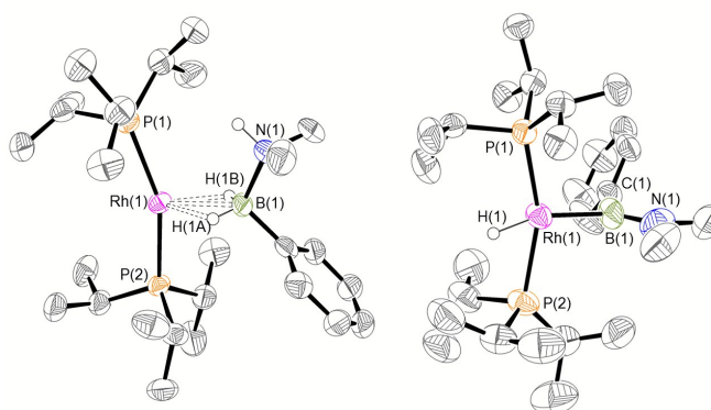
Figure 4: X-ray molecular structures of [\text{RhH}_2(\text{P}^i\text{Pr}_3)_2(\eta^2\text{-H}_2\text{PhB}\cdot\text{NMe}_2\text{H})][\text{BARF}_4] (10), left, one independent cation from the asymmetric unit is shown; and [\text{RhH}(\text{P}^i\text{Pr}_3)_2(\text{BPhNMe}_2)][\text{BARF}_4] (11), right. [\text{BARF}_4]^- anions, minor components of disorder and selected H atoms omitted for clarity. Ellipsoids shown at 50% probability level. Selected bond lengths (Å) and angles (°). (10) [values are also given for the second cation in the asymmetric unit which is not shown in the figure]: Rh(1)–P(1) 2.336(2), Rh(1)–P(2) 2.330(2), Rh(1)–B(1) 2.274(9), B(1)–N(1) 1.650(11), Rh(2)–P(3) 2.3227(19), Rh(2)–P(4) 2.327(2), Rh(2)–B(2) 2.333(8), B(2)–N(2) 1.608(11); P(1)–Rh(1)–P(2) 158.35(8), P(3)–Rh(2)–P(4) 155.75(8). (11): Rh(1)–P(1) 2.3292(18), Rh(1)–P(2) 2.350(2), Rh(1)–B(1) 1.929(9), B(1)–C(1) 1.536(14), B(1)–N(1) 1.411(14); P(1)–Rh(1)–P(2) 157.55(7), P(1)–Rh(1)–B(1) 100.2(3), P(2)–Rh(1)–B(1) 100.6(3), Rh(1)–B(1)–N(1) 138.0(8), Rh(1)–B(1)–C(1) 98.3(7), N(1)–B(1)–C(1) 123.7(8)
