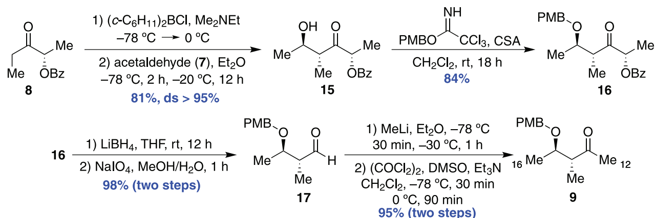
Scheme 3. Synthesis of \alpha -methyl- \beta -hydroxyketone 9 .
