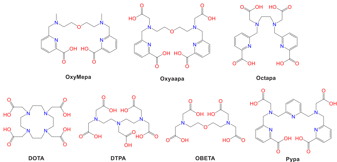
Chart 1. Chemical Structures of the Chelators Discussed in This Work
