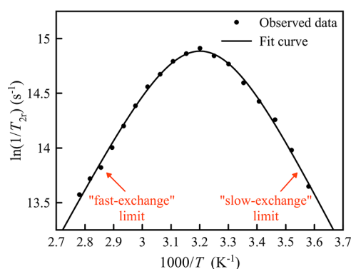
Figure 4. Temperature dependence of the reduced transverse ^{17}\text{O} relaxation rate of 3.0 mM Gd-OxyMepa complex (pH = 7.4 in 0.1 M MOPS).
