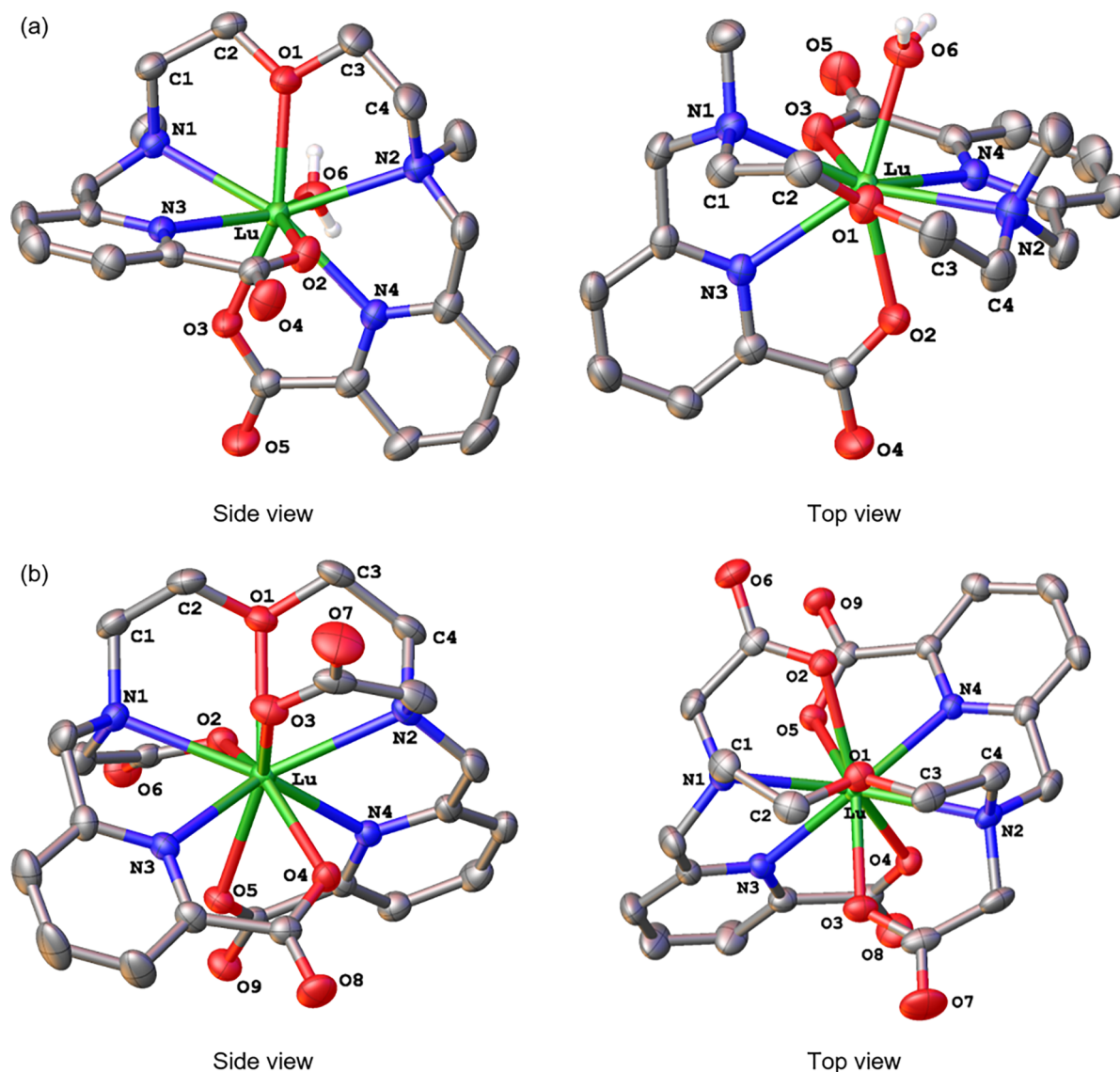
Figure 1. Crystal structures of (a) Lu-OxyMepa and (b) Lu-Oxyaapa. Thermal ellipsoids are drawn at the 50% probability level. Solvent, counterions, and nonacidic hydrogen atoms are omitted for clarity.
