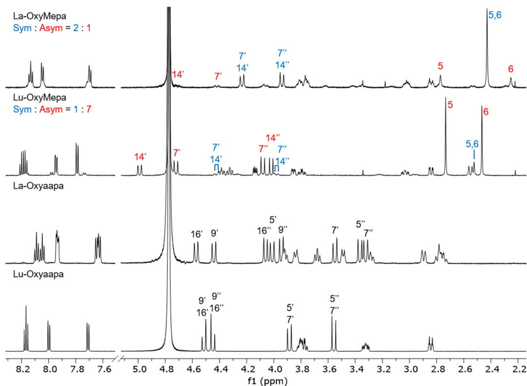
Figure 2. ^1\text{H} NMR spectra of OxyMepa and Oxyaapa complexes formed with \text{La}^{3+} and \text{Lu}^{3+} (600 MHz, \text{D}_2\text{O} , \text{pD} = 7 , 25^\circ\text{C} ). Diagnostic peaks are labeled, and the numbering scheme is shown in Chart 2. The high-intensity peak near 4.8 ppm arises from residual HDO in the NMR solvent.
