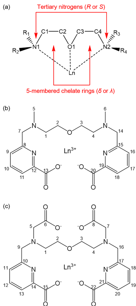
Chart 2. (a) Depiction of the Sources of Chirality in Ln-OxyMepa or Ln-Oxyaapa Complex; (b) Numbering Scheme of Ln-OxyMepa Complex; (c) Numbering Scheme of Ln-Oxyaapa Complex
